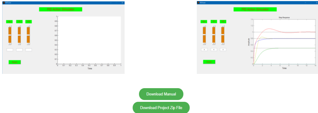
Fig 3: Application 1 page
