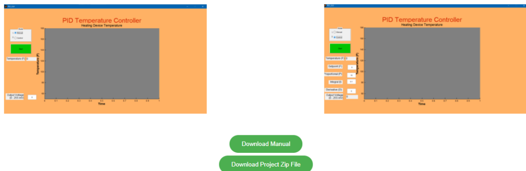
Fig 4: Application 2 page
